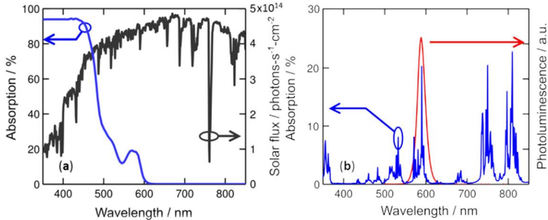
Figure 2 (a) Absorption of the luminescent colloidal film, 10% wt. CdSe/CdZnS:PVB-CVACVAc (blue), overlaid on the AM1.5 solar flux (black). (b) The luminescence of the nanocrystal (red) is tuned to an absorption peak of the Nd 3+ :YAG (blue), for efficient waveguided luminescent pumping of optical gain media [19].
