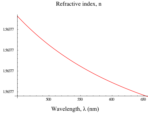
Figure. 2: The refractive index of the liquid crystal (E7) as a function of wavelength between 450-656 nm [3].
