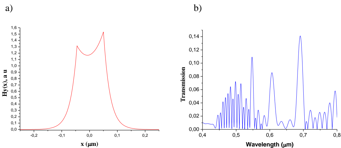
Figure 6 (a) Surface plasmon magnetic field profile of silver-E7-silver guide ( \lambda=633\text{nm} , 2w=0.1 \mu\text{m} ), and (b) the transmission spectrum.
