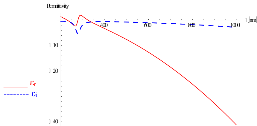
Figure.1: The real and imaginary components of the permittivity of Ag
