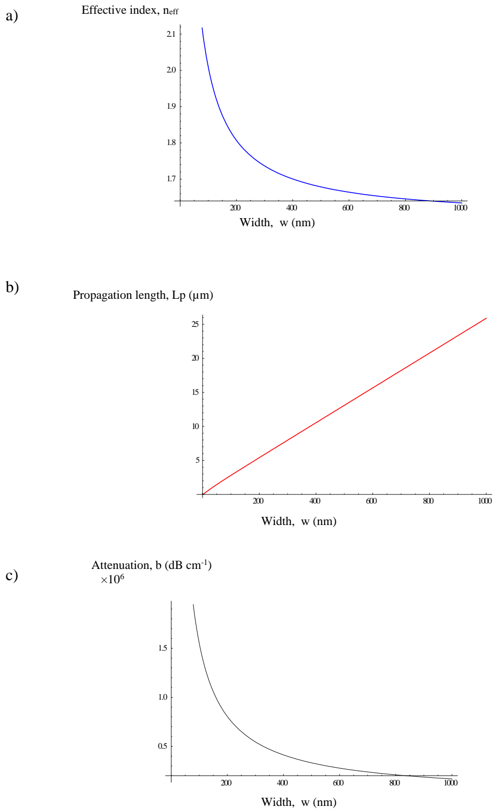
Figure 4 The effective index n_{eff} , propagation length L_p , and the attenuation b , as functions of width of the gap of the E7 w for \lambda=633\text{ nm} (MIM plasmonic waveguides Ag/E7/Ag, \epsilon_d = 2.5363 and silver metal \epsilon_{Ag} = -14.4688 - i 1.09378 .)
