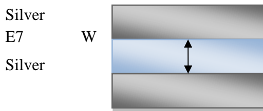
Figure 3 Schematic of MIM plasmonic waveguide.
