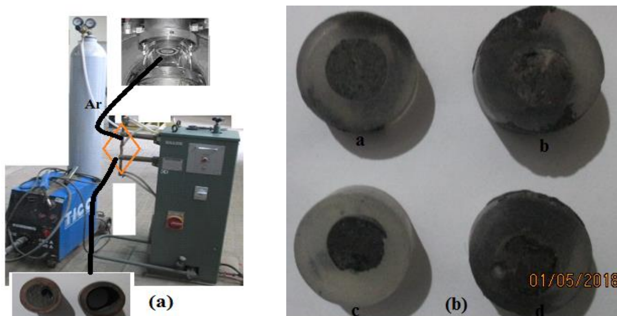
Figure 1 Schematic representation of ETE-VC chamber and produced samples (b).
