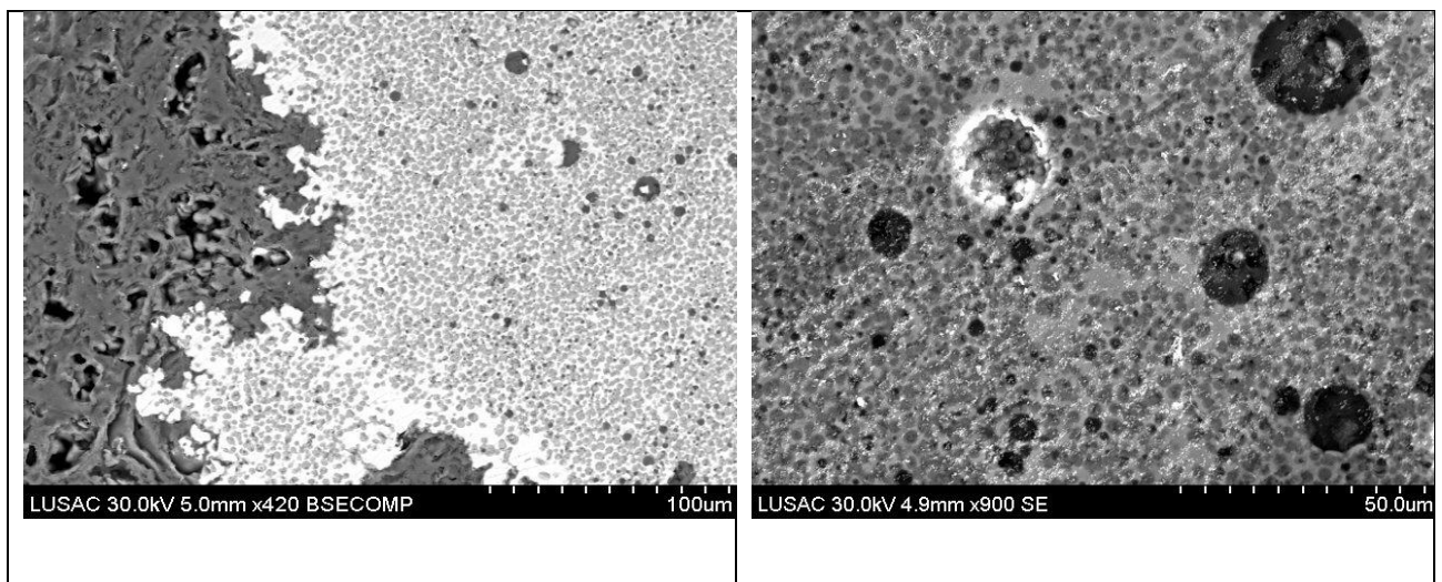
Figure 2a FESEM microstructures of polished and etched surface of samples with 10 wt.% Fe.
