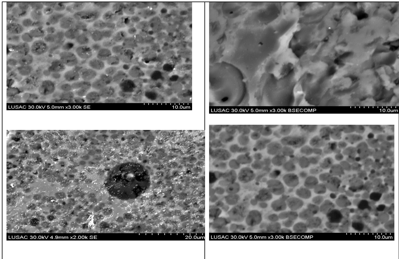
Figure 2b FESEM microstructures of polished and etched surface of samples with 20 wt.% Fe.
