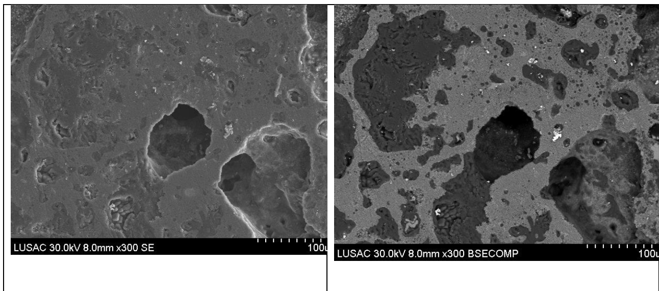
Figure 2b FESEM microstructures of polished and etched surface of samples with 20 wt.% Fe.
