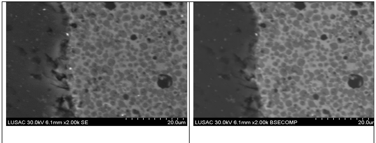
Figure 2a FESEM microstructures of polished and etched surface of samples with 10 wt.% Fe.
