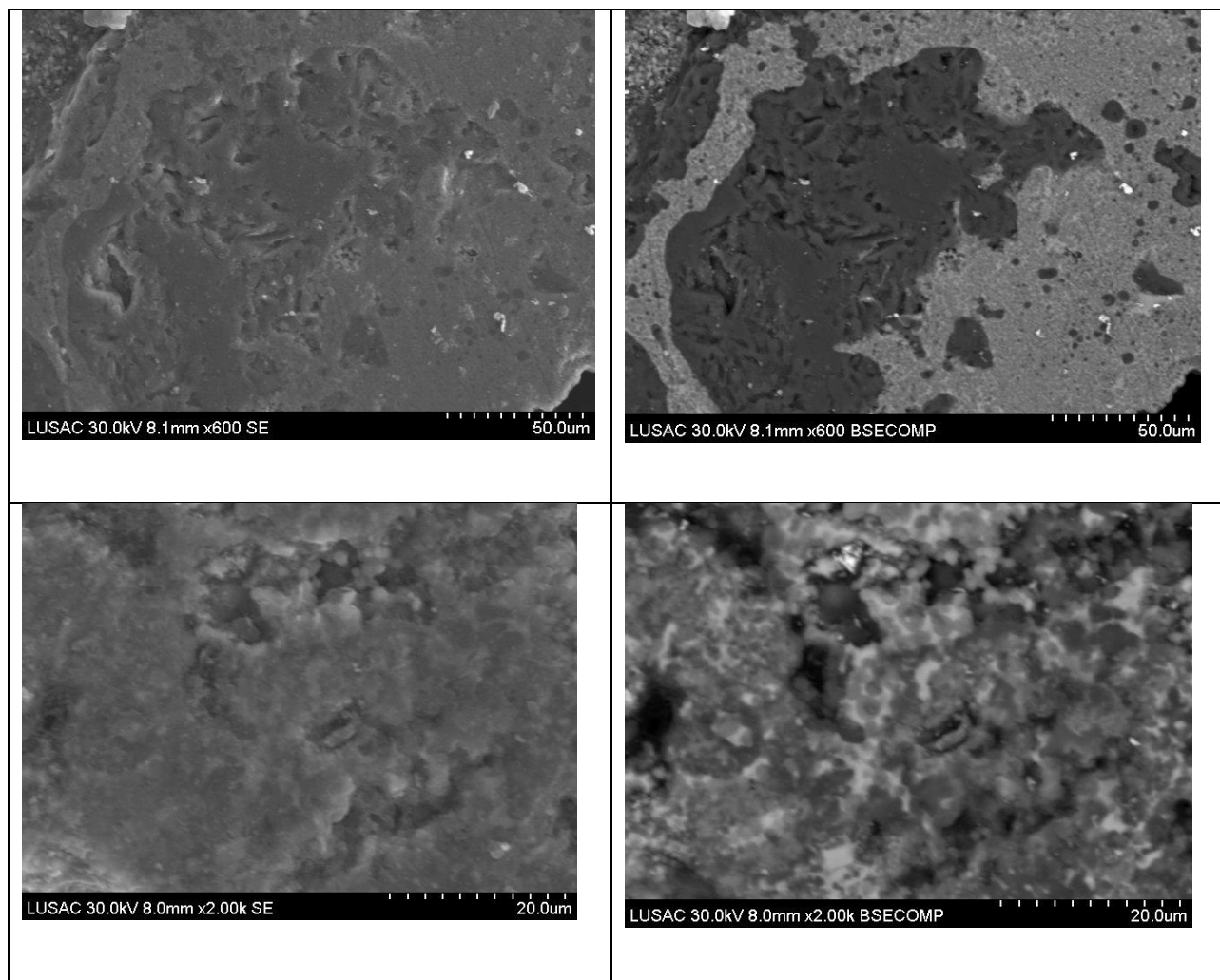
Figure 3c FESEM microstructures of polished and etched surface of samples with 40 wt.% Fe.
