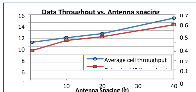
Figure 10 average cell throughput and cell-edge user throughput vs. antenna element spacing.
