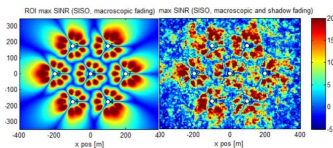
Figure 4 SINR mapping, BBUs each with three RRHs having directional antennas, left is path loss map and right is path loss plus shadowing map.
