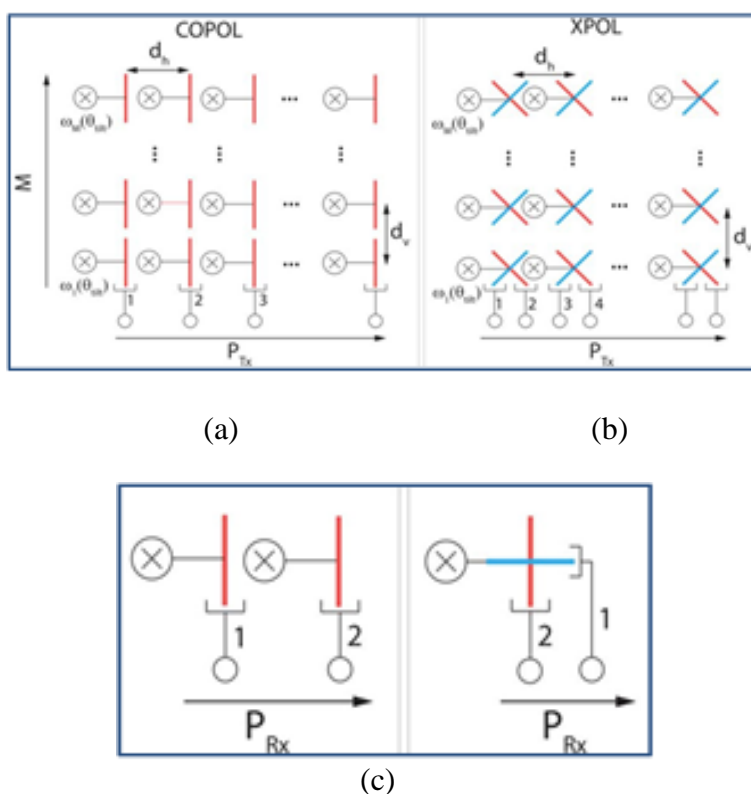
Figure.8 Antenna configuration and polarization modes at (a,b) base station antenna array and (c) UE antenna.
