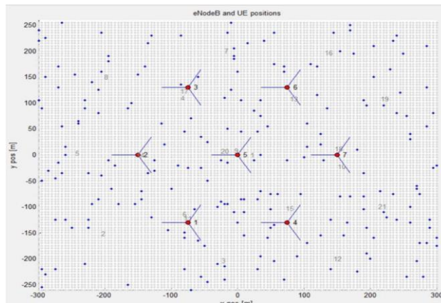
Figure 9 5G nodes & UE map with 150m inter-node-distance, and 210 UEs (dark dots) with 10 UEs per cell
