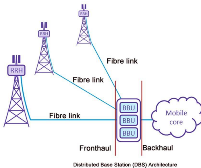
Figure 1 Distributed Base Station Architecture.
