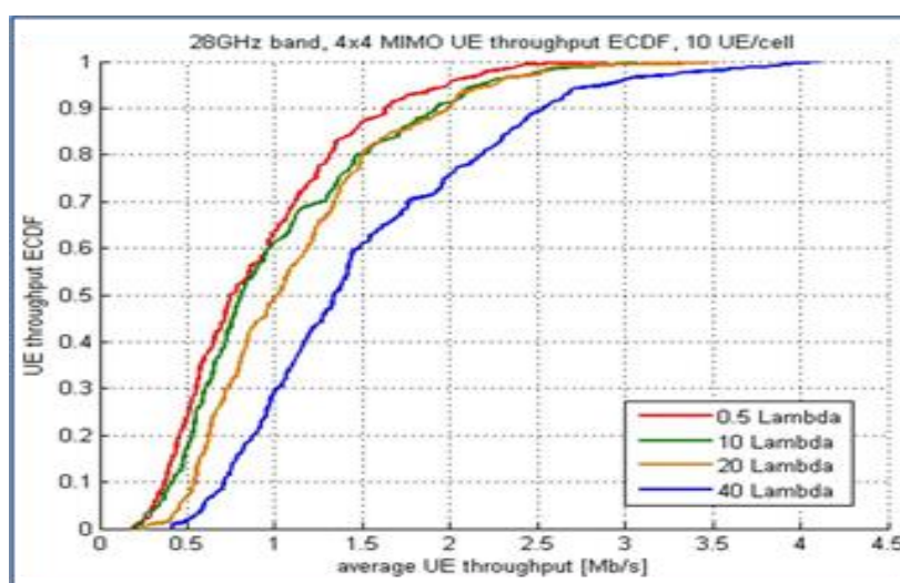
Figure 11 average UE throughput for multiple antenna element spacing.
