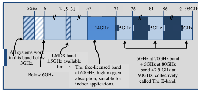
Figure 3 Millimetre-wave band as a candidate spectrum to 5G
