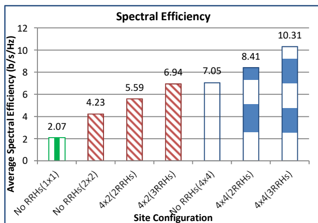
Figure.5 average spectral efficiency (p/s/Hz)
