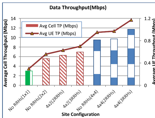
Figure 6 average cell and UE data throughput (Mbps)
