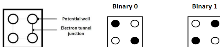
Figure 1 Basic QCA Cell and possible alignments of electrons
