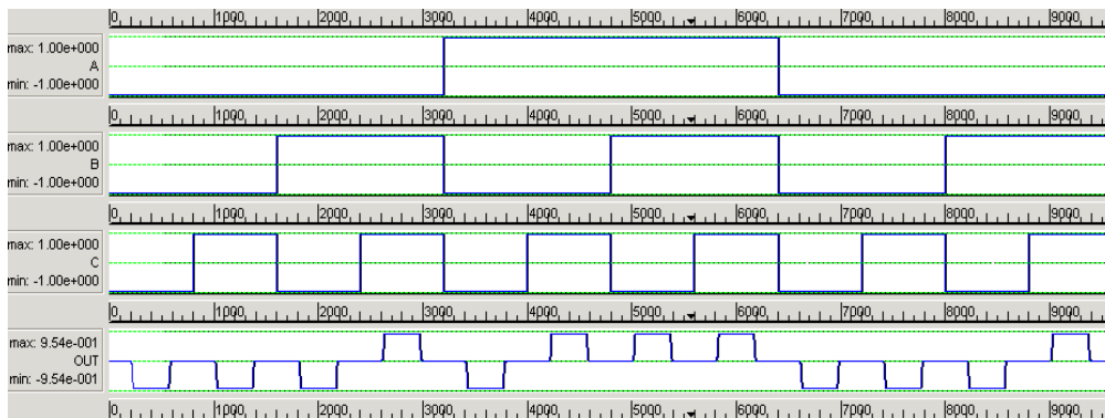
Figure 8 Majority Voter Implementation and simulation results in QCA Designer 2.0.3
