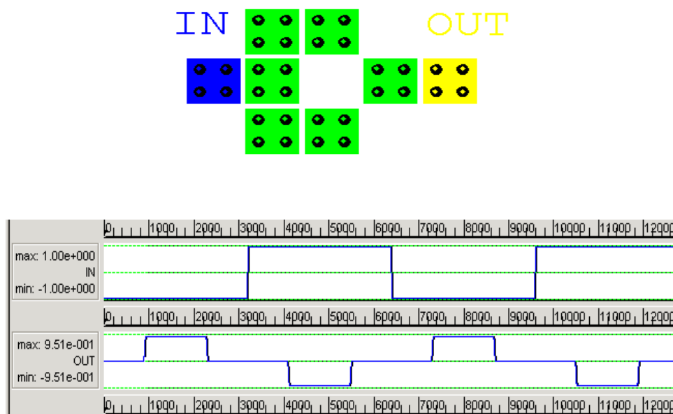
Figure 6 Inverter Implementation and simulation results in QCA Designer 2.0.3
