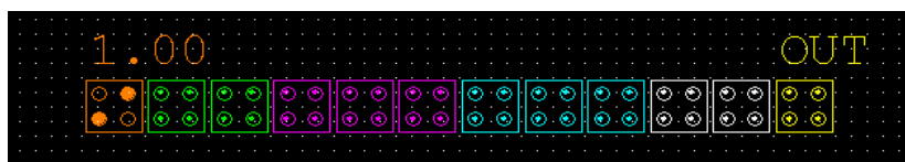
Figure 12 Clocked QCA wire
