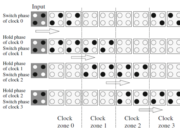
Figure 11 Illustration of clocking in QCA Cells
