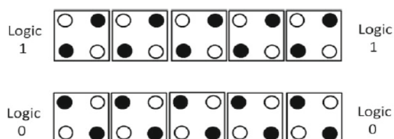
Figure 3 Binary Wire
