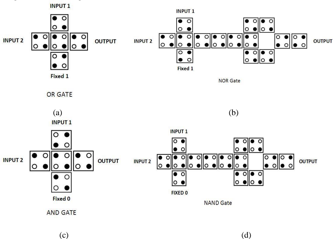
Figure 9 (a) OR Gate (b) NOR Gate (c) AND Gate (d) NAND Gate implementation using majority gate
