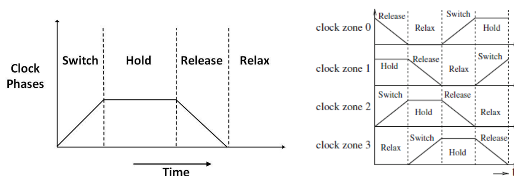
Figure 10 Different Clock Phases and clock zones in QCA
