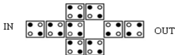
Figure 5 QCA Inverter
