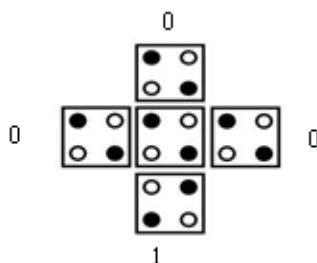
Figure 7 QCA Majority Voter
