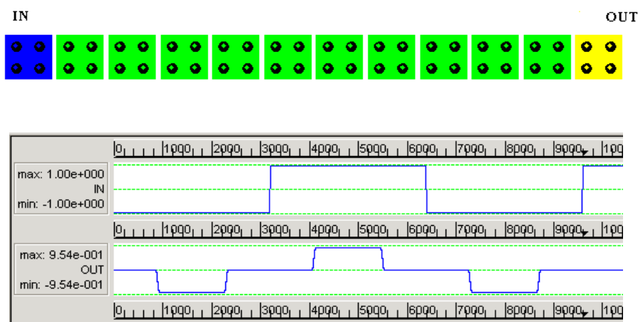
Figure 4 Binary wire implementation and simulation result in QCA Designer 2.0.3
