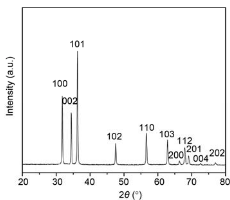
Figure 3 XRD pattern of the ZnO microcrystals.
