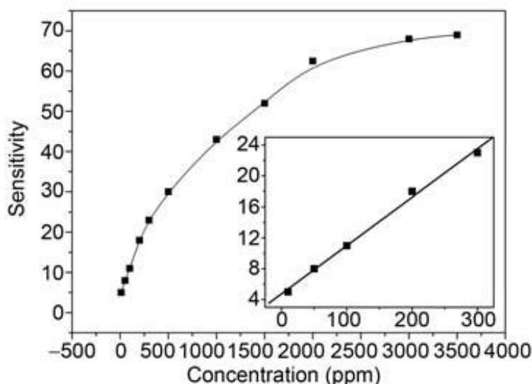
Figure 6 The sensitivity of the ZnO microcrystal sensor vs. ethanol concentration. The insert is the calibration curve in the range of 1–300 ppm.
