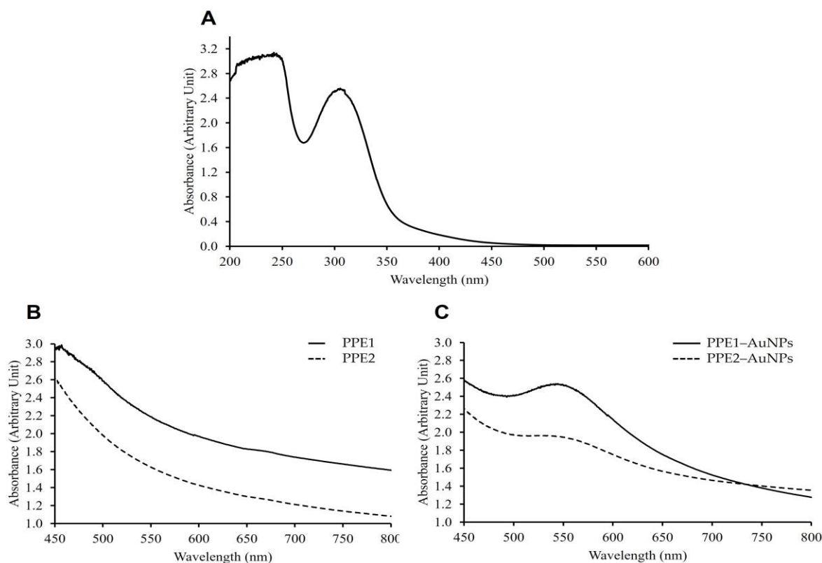
Figure 3 UV–Visible spectra of HAuCl 4 , pomegranate peel extracts, and green-synthesized AuNPs. (A) Spectrum of 1 mM HAuCl 4 showing a characteristic absorption band at approximately 310 nm and no absorption in the visible region. (B) UV–Vis spectra of PPE1 (air-dried) and PPE2 (oven-dried) extracts, exhibiting strong ultraviolet absorption have associated with phenolic compounds but no SPR band. (C) UV–vis spectra of PPE1–AuNPs and PPE2–AuNPs showing characteristic SPR bands of AuNPs, with PPE1–AuNPs exhibiting a sharper, more intense peak ( \lambda_{\text{max}} \approx 555 nm) than PPE2–AuNPs.
