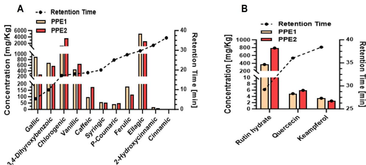
Figure 1 Phenolics and flavonoids in Omani pomegranate peel extracts are determined by UPLC-DAD. Phenolic acids (A) and flavonoids (B) in PPE1 (air-dried) and PPE2 (oven-dried), are reported as concentrations (mg/kg extract); dotted line shows retention time (min).
