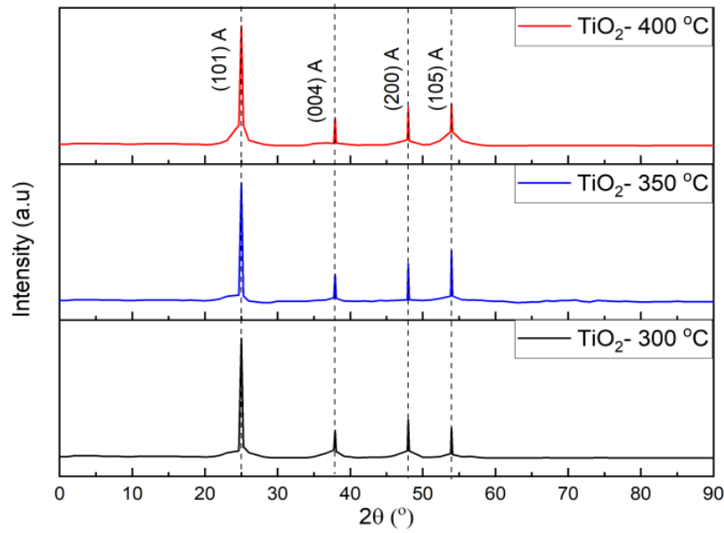
Figure 10 XRD spectra of TiO 2 thin films with 300, 350 and 400 °C.
