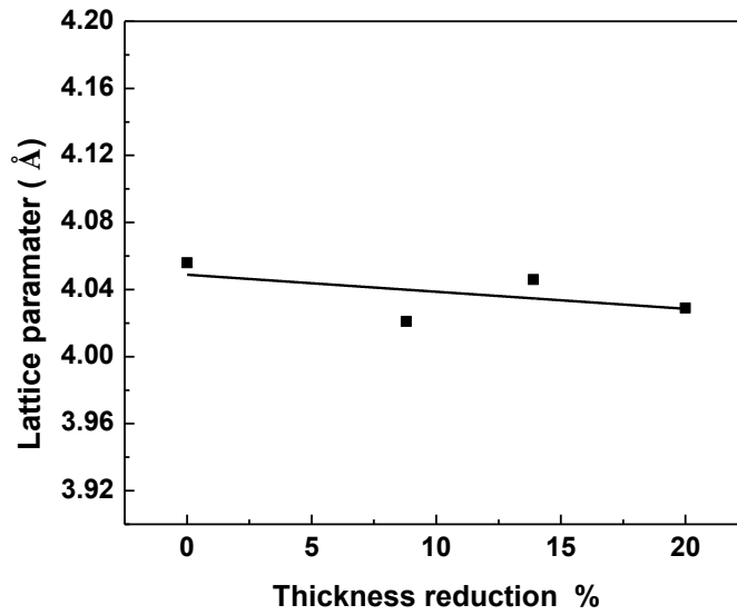
Figure 2 Lattice parameter as a function of thickness reduction of 1070 al Alloy.
