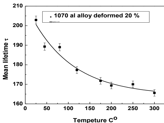
Figure 5 The mean lifetime as a function of annealing Temperature.
